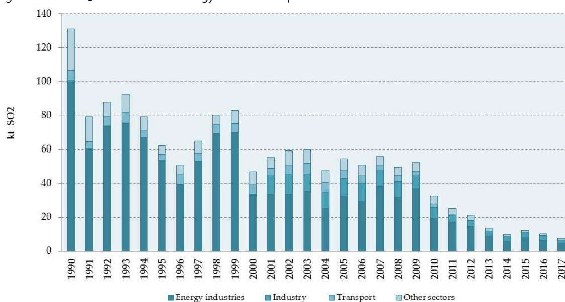
Figure 3.1-11: SO 2 emissions from Energy sector in the period 1990-2017
