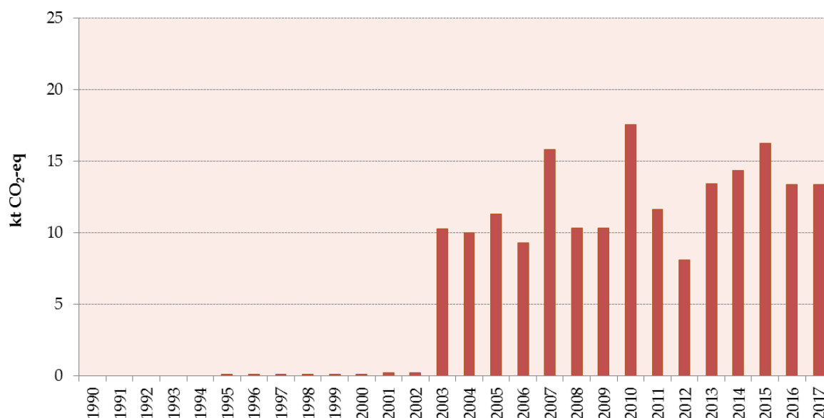
Figure 4.7-2: Emissions of HFCs used in 2.F.2, 2.F.3 and 2.F.4 (kt CO 2 -eq), (1990 - 2017)
