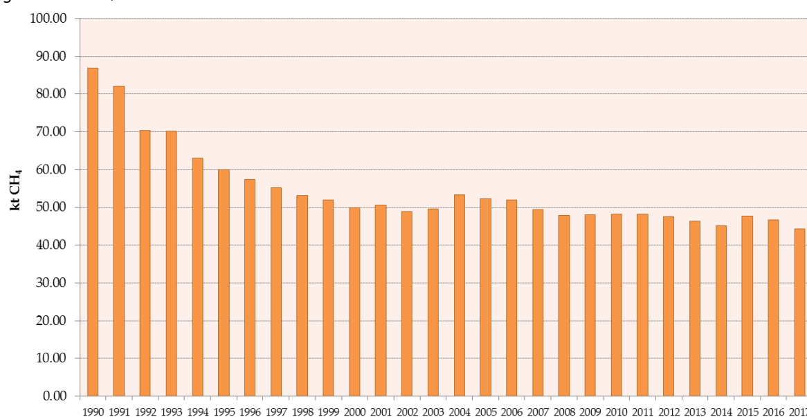
Figure 5.2-1: CH 4 emission from Enteric fermentation
