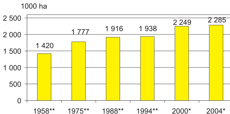
Figure 1.4.1.1 Changing of forest land area
