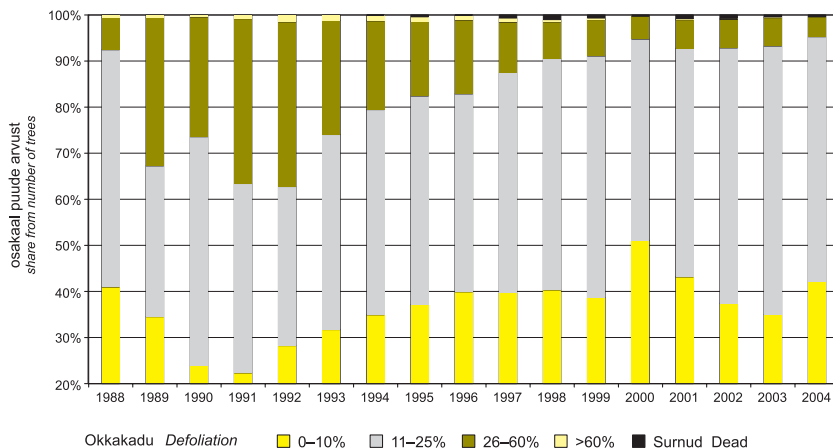
Joonis 5.6.1 Hariliku männi okkakadu metsaseire proovipunktides aastail 1988–2004 Figure 5.6.1 Defoliation of Scots pine on forest monitoring sample points in 1988–2004
