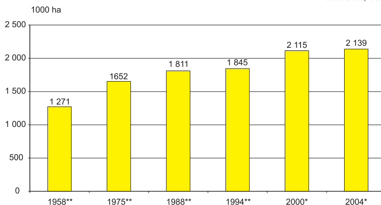
Figure 1.5.1.1 Changing of area of stands
