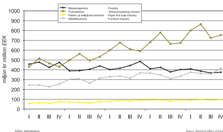
Figure 10.1.2.2 Changing of added value of forest sector companies at year 2000 constant prices in 2000–2004 (year 2000=100%)
