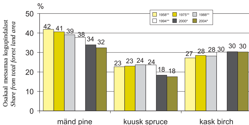
Figure 1.4.1.2 Changing of share of tree species
