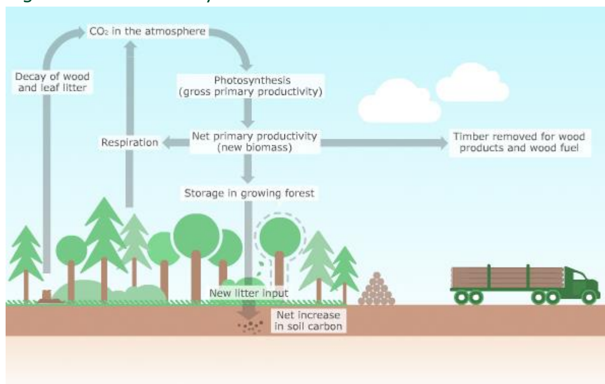
Figure 4.1 Carbon Cycle
